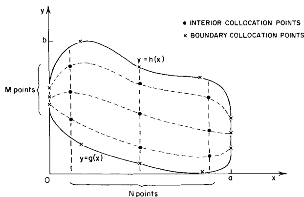
Fig. 1. Two-dimensional arrangement of collocation points for an irregular domain, \cdot interior collocation points, \times boundary collocation points.
